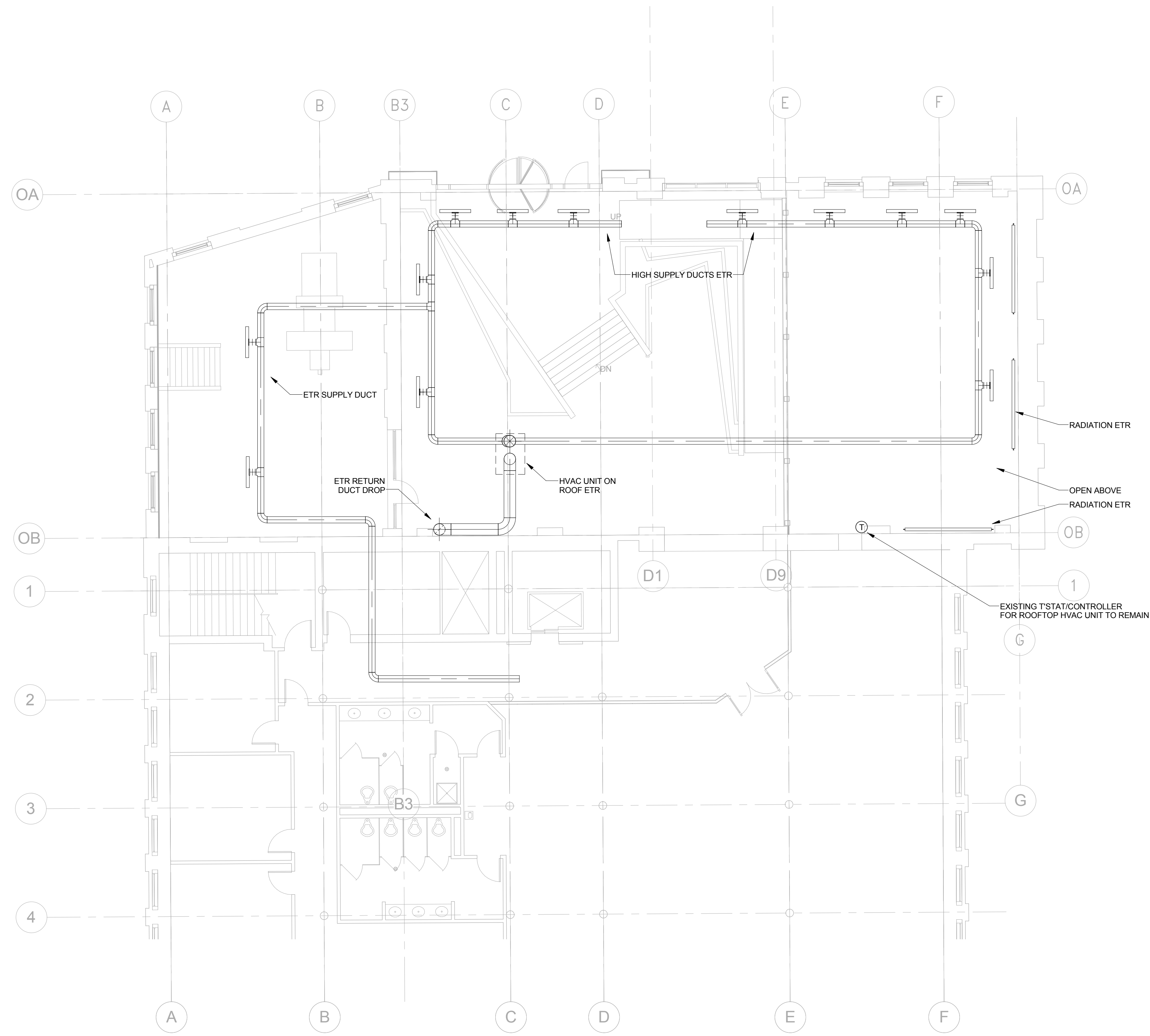
① Building 5 - Level 1 - HVAC DUCTWORK & PIPING 1/8" = 1'-0"
