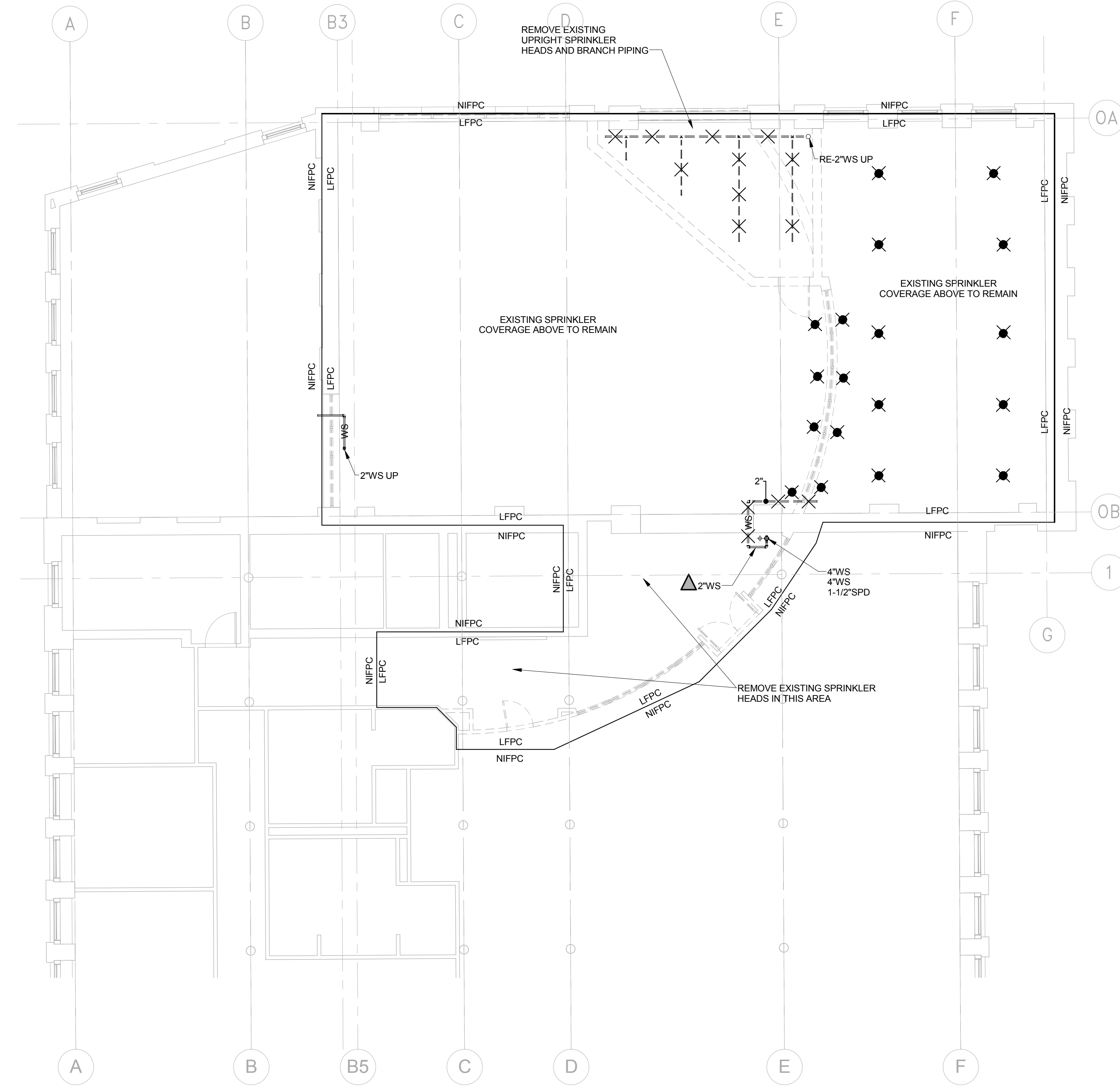
1 Building 5 - Level 1 Demo - Fire Protection 1/8" = 1'-0"
