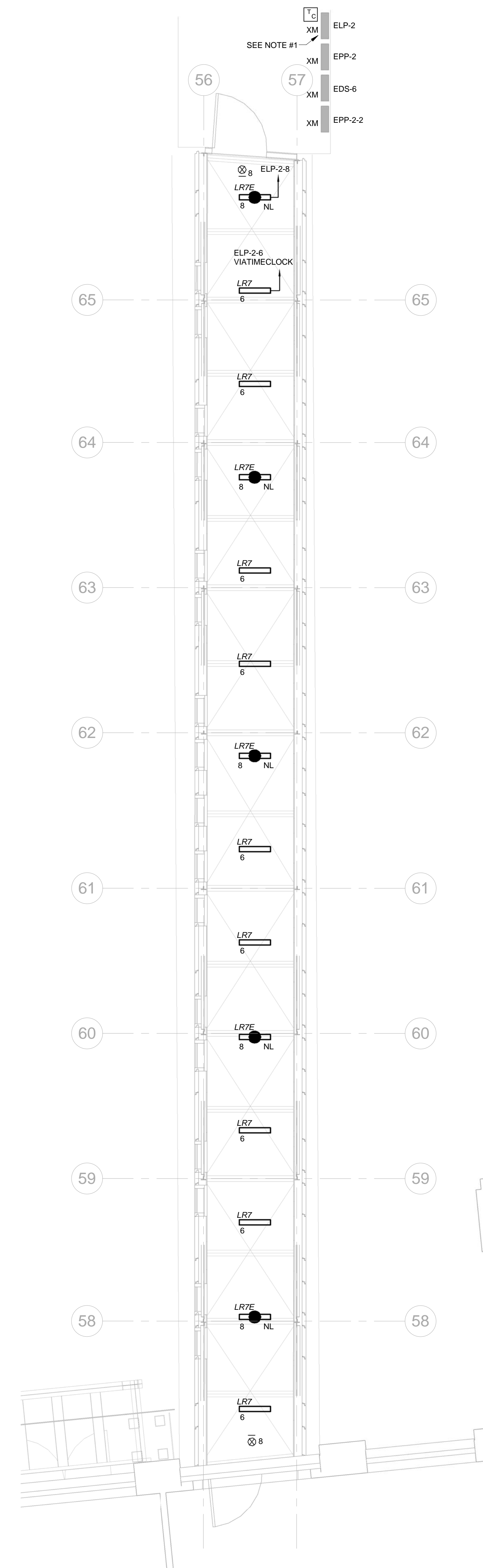
1 BUILDING 3 - ELECTRICAL LIGHTING BRIDGE A PLAN 1/4" = 1'-0"
