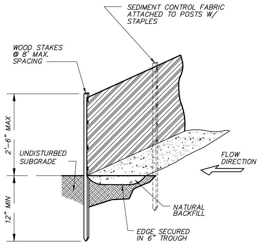
SILTATION FENCE DETAIL NOT TO SCALE
