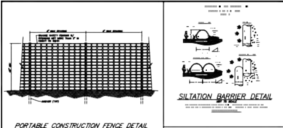
PORTABLE CONSTRUCTION FENCE DETAIL NOT TO SCALE
