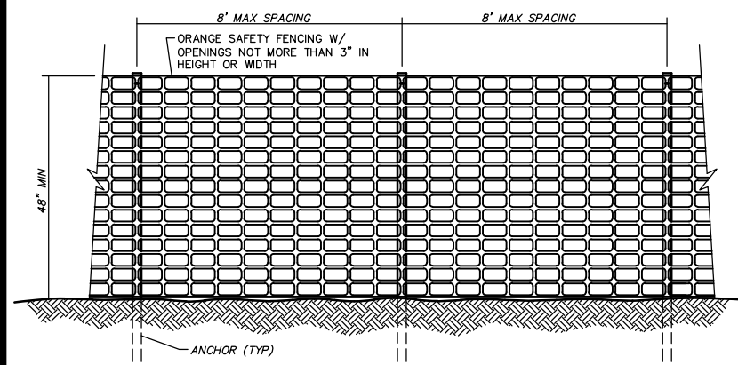
PORTABLE CONSTRUCTION FENCE DETAIL NOT TO SCALE
