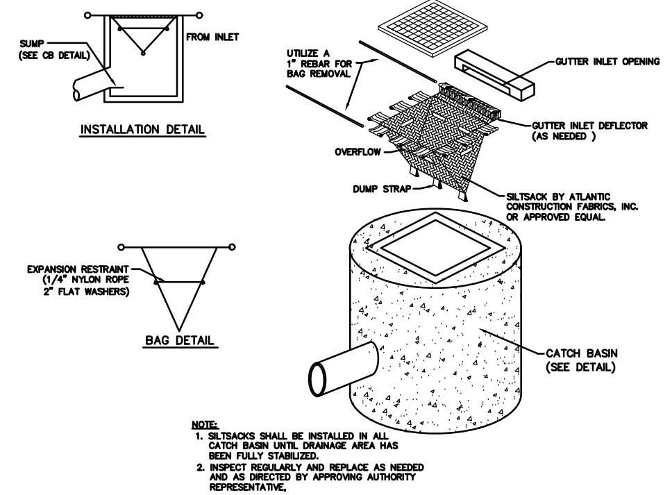
EROSION CONTROL SILT SACK DETAIL NOT TO SCALE
